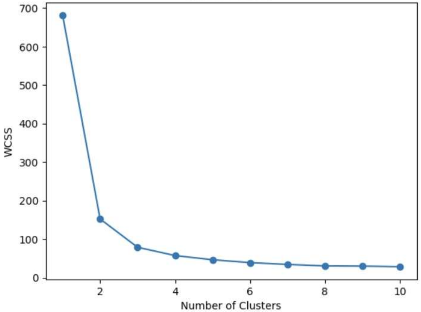
Elbow Method
