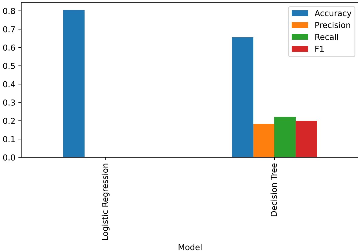
RQ5 Metric Sensitivity
