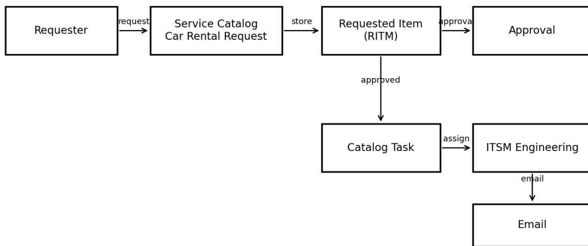
Figure 1: Architecture and data flow of the Car Rental Request Automation solution
