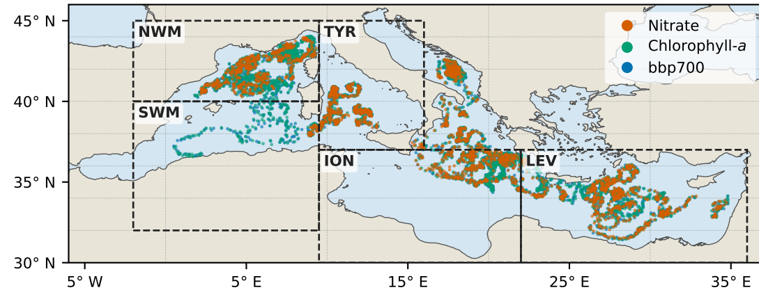
Train
