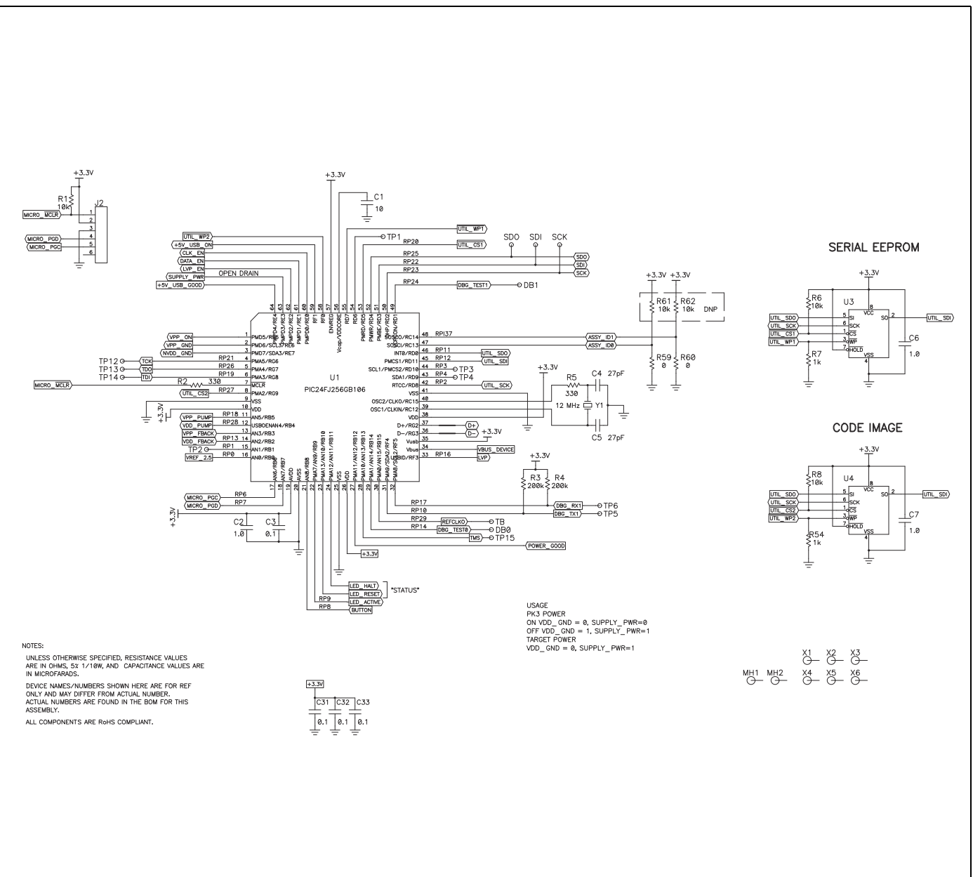
FIGURE B-1: PICKit™ 3 SCHEMATIC DIAGRAM (PAGE 1 OF 2)
