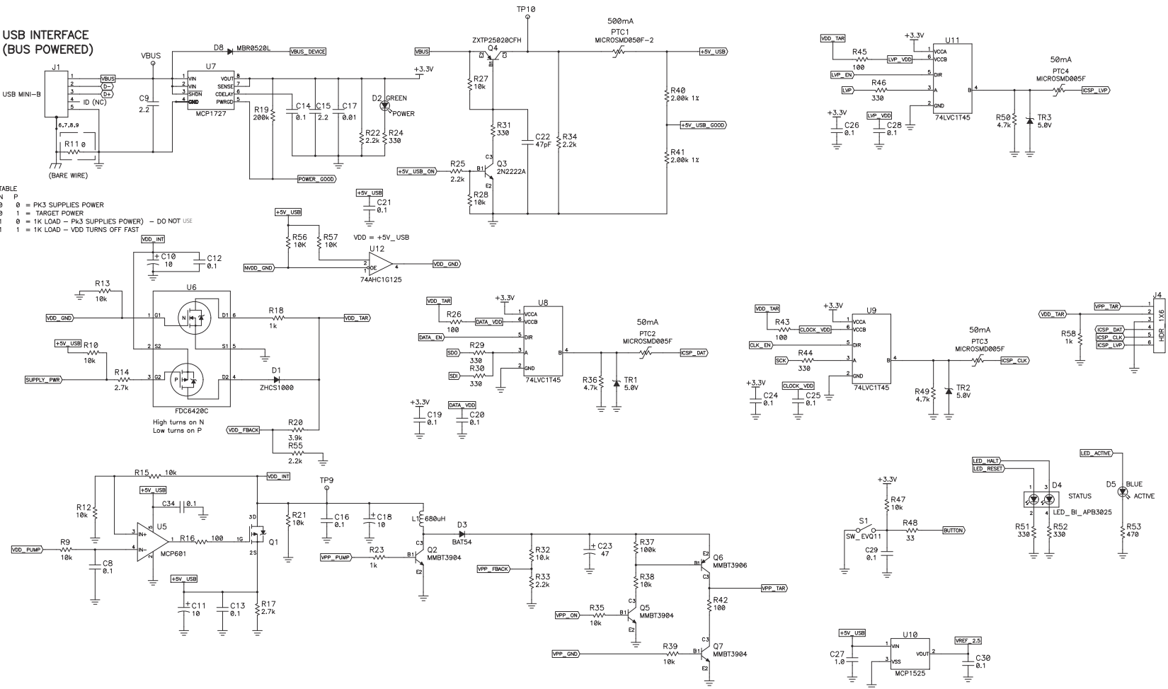
FIGURE B-2: PICKit™ 3 SCHEMATIC DIAGRAM (PAGE 2 OF 2)
