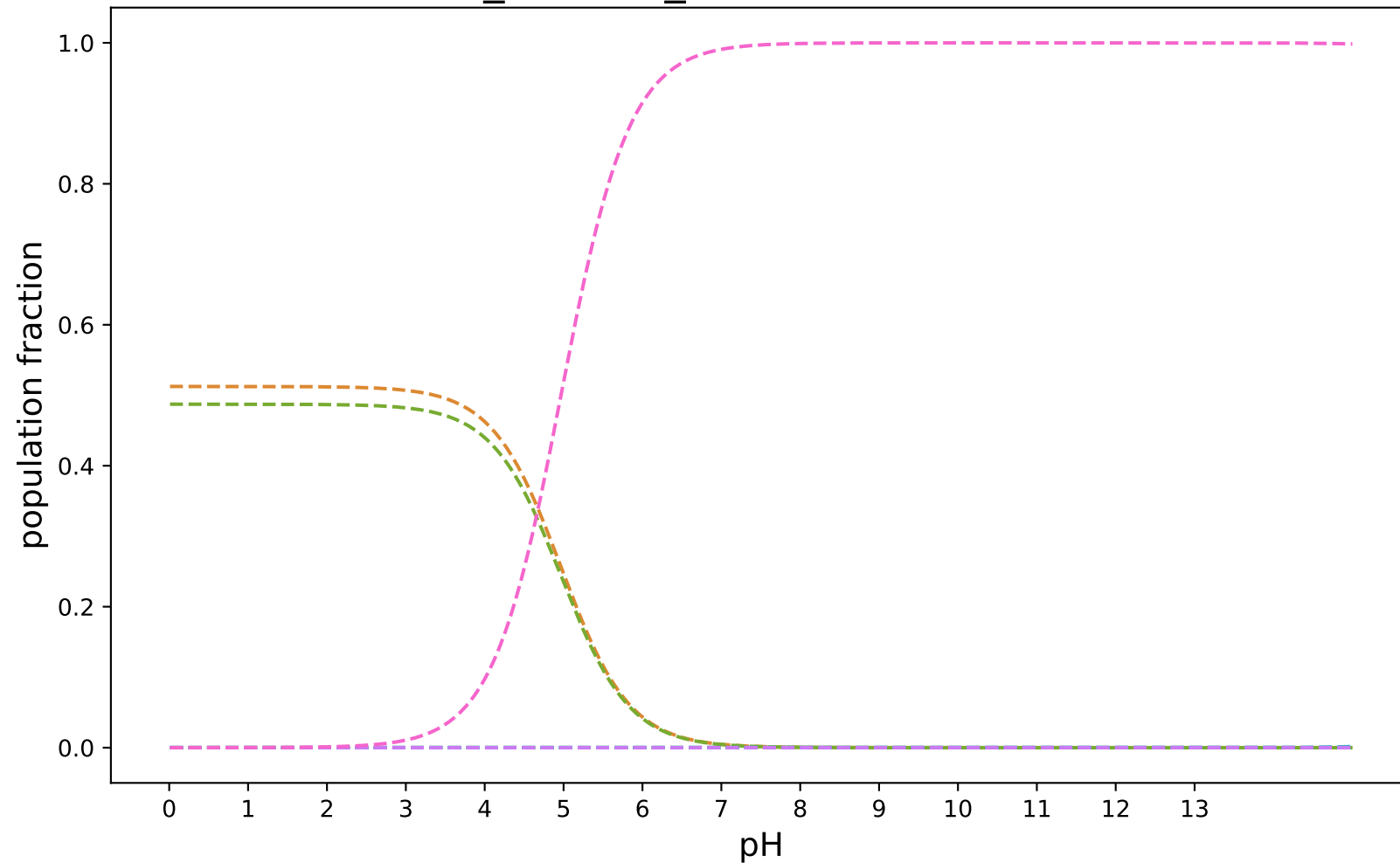
PKA_ECRISM_modified:SAMPL8-12
