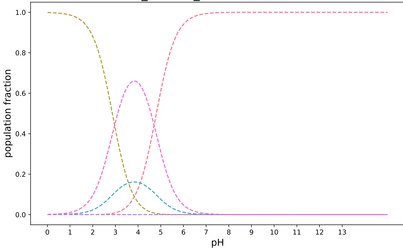
PKA_ECRISM_modified:SAMPL8-6
