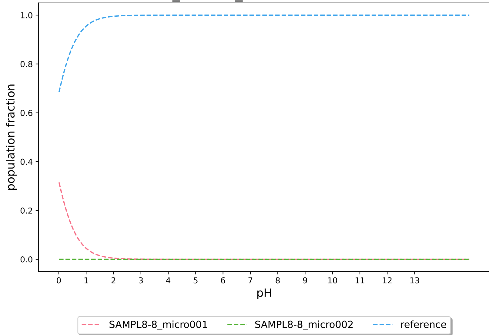
PKA_ECRISM_modified:SAMPL8-8
