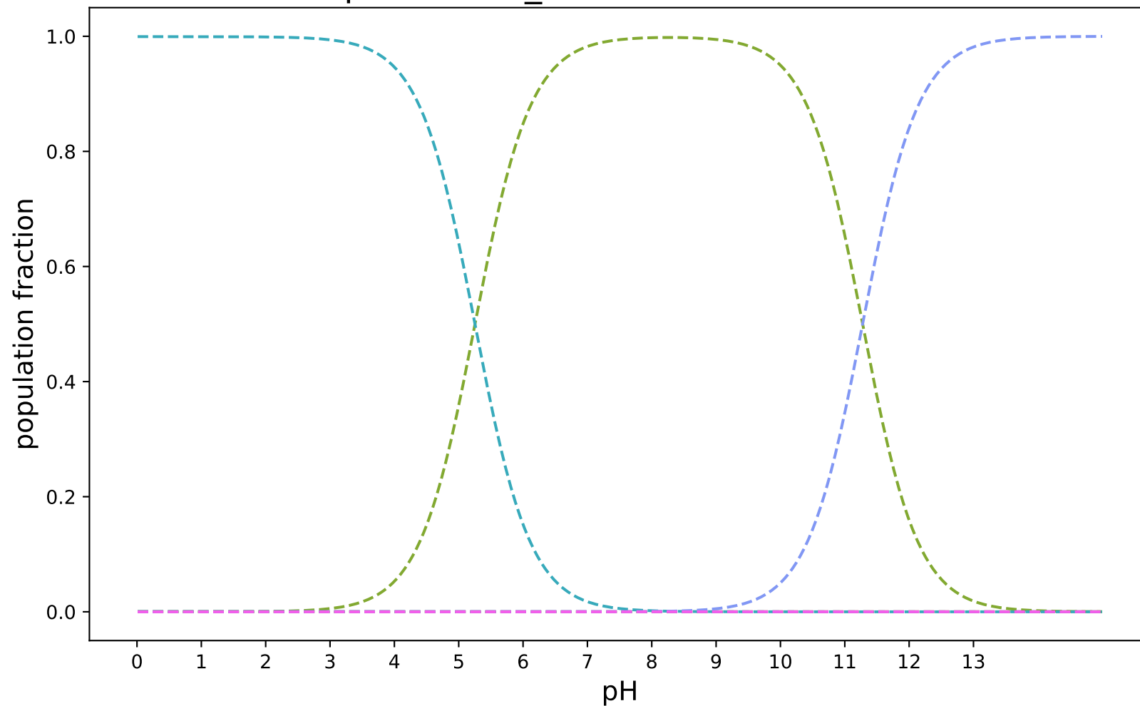
pKa-3DS-1_modified:SAMPL8-18
