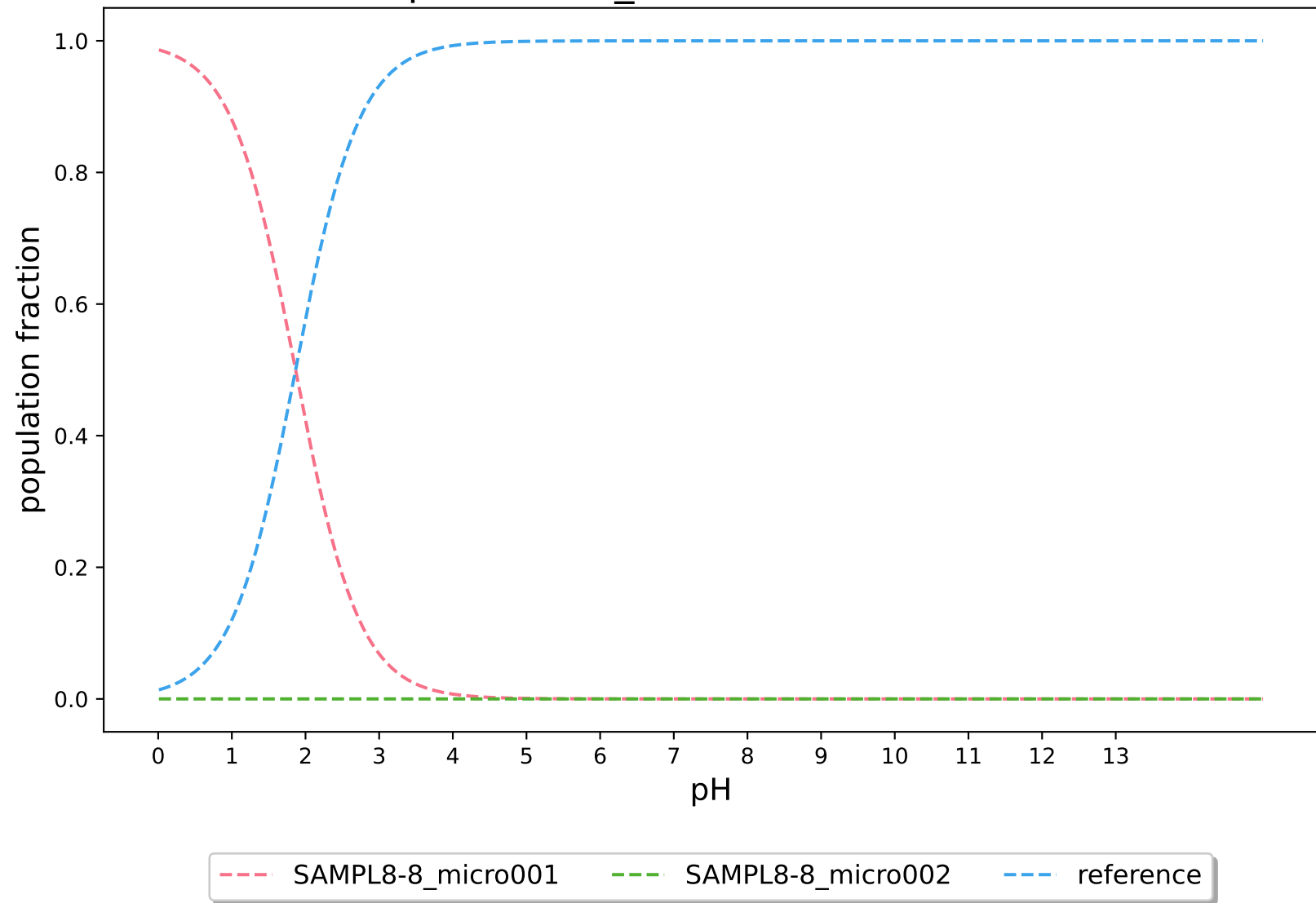
pKa-3DS-1_modified:SAMPL8-8
