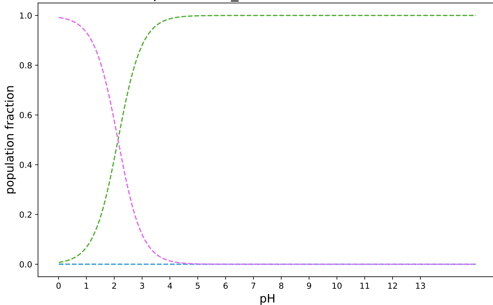
pKa-3DS-2_modified:SAMPL8-1
