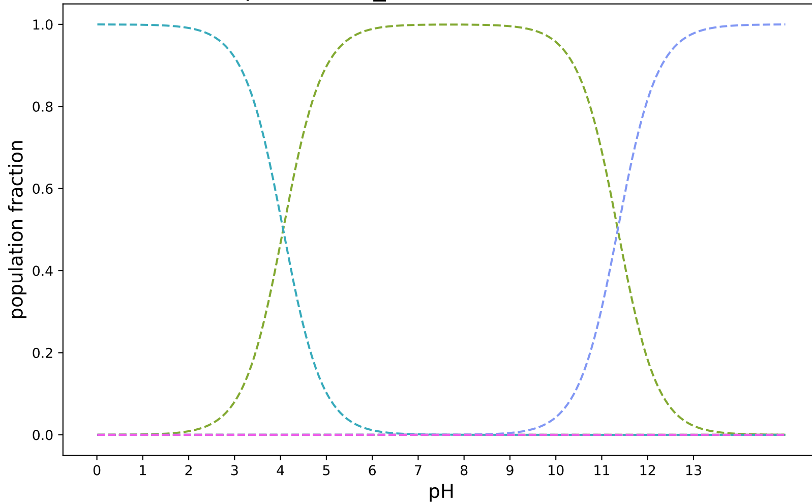
pKa-3DS-2_modified:SAMPL8-18
