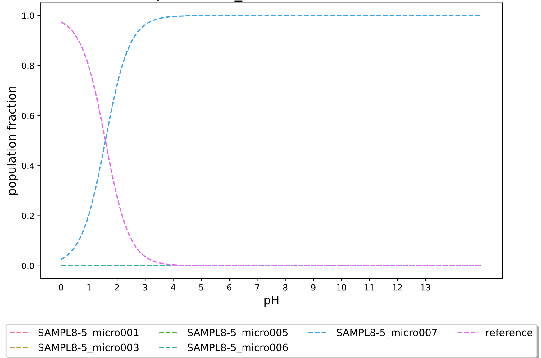
pKa-3DS-2_modified:SAMPL8-5
