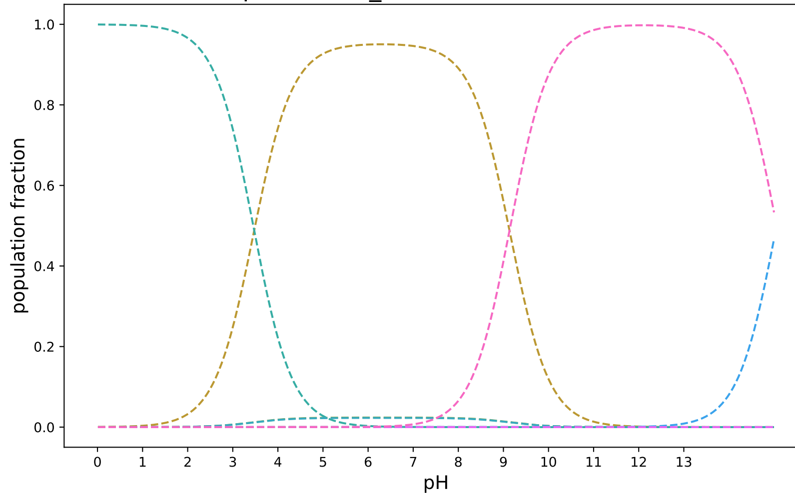
pKa-3DS-3_modified:SAMPL8-12
