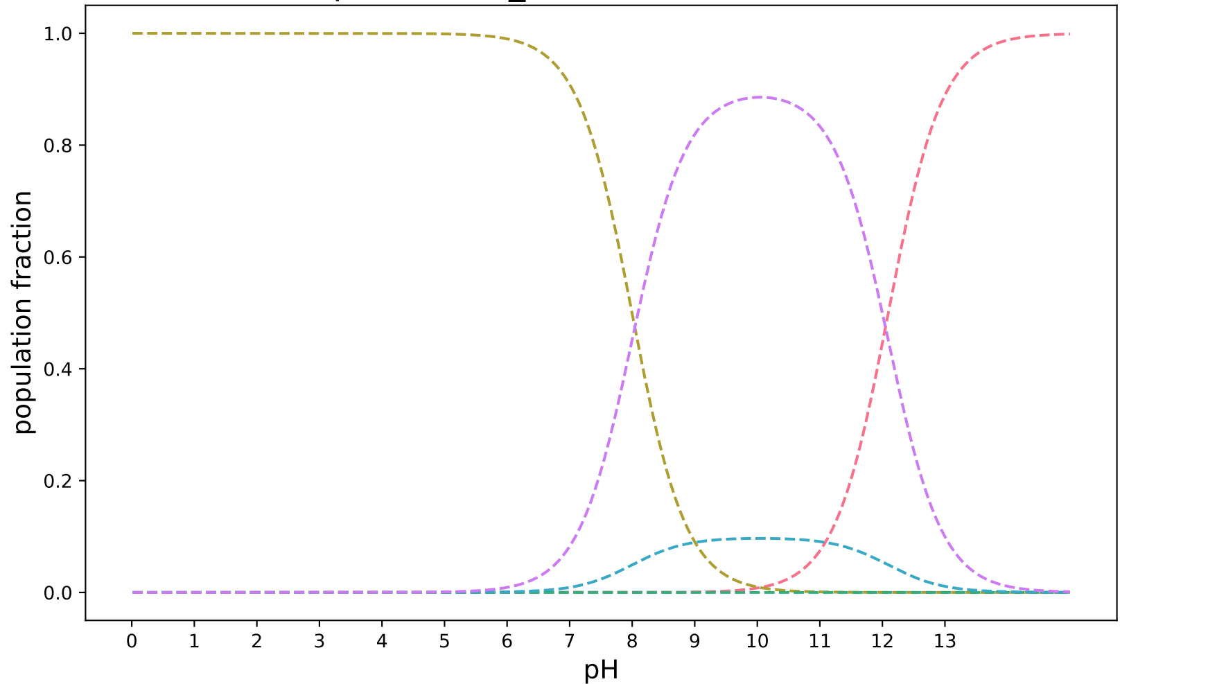
pKa-3DS-3_modified:SAMPL8-17
