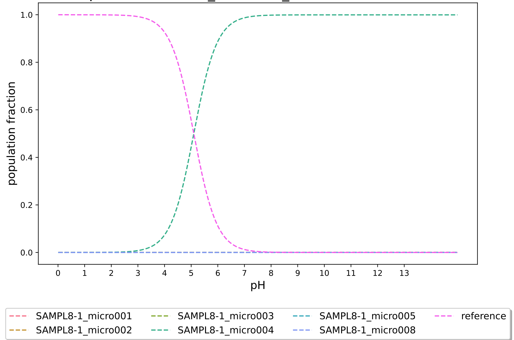
pKa-RobertRaddi_AdaBoost_modified:SAMPL8-1
