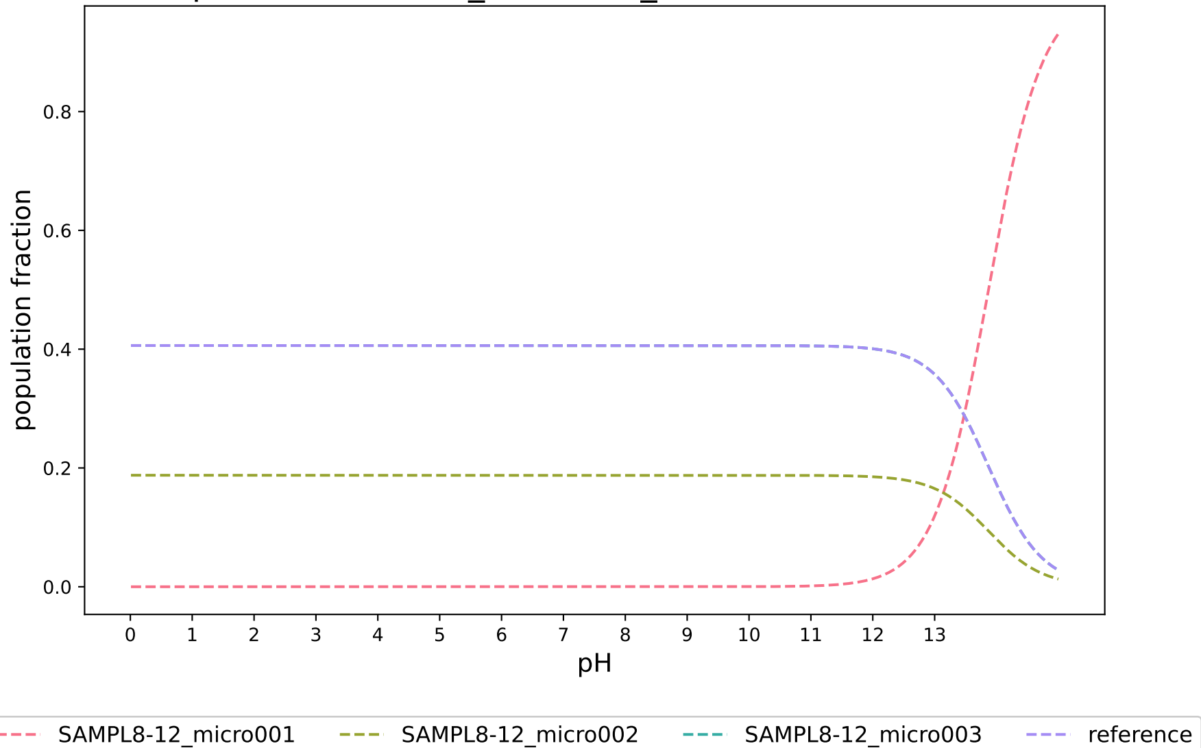
pKa-RobertRaddi_AdaBoost_modified:SAMPL8-12
