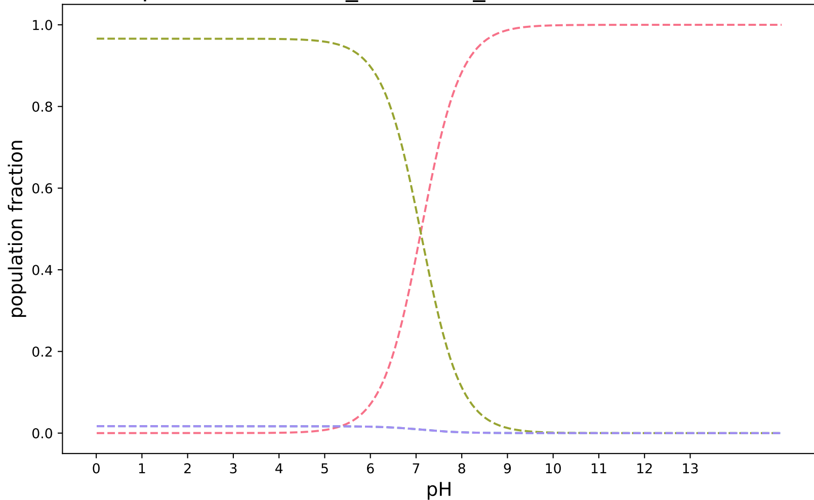
pKa-RobertRaddi_AdaBoost_modified:SAMPL8-22
