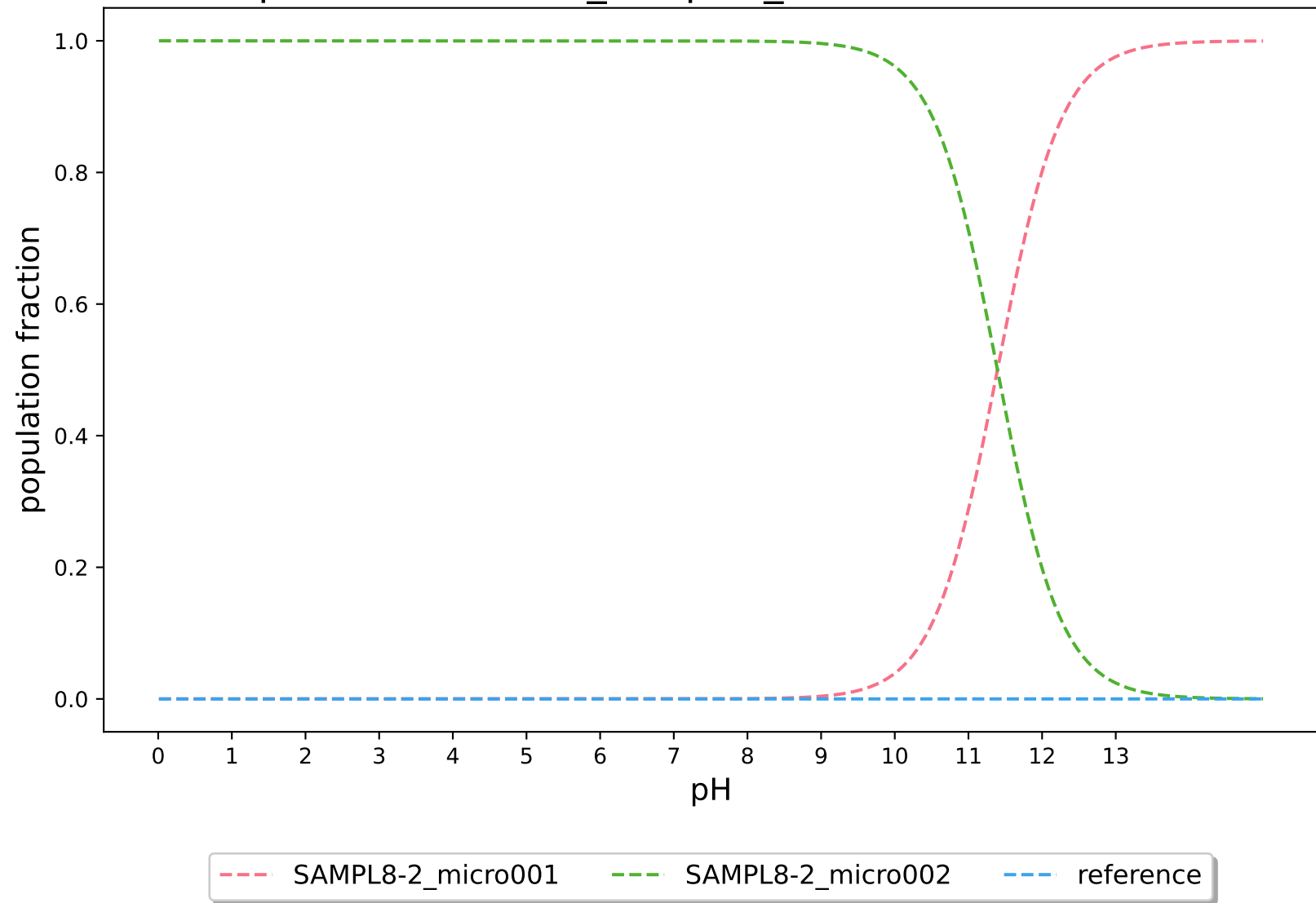
pKa-RobertRaddi_DeepGP_modified:SAMPL8-2
