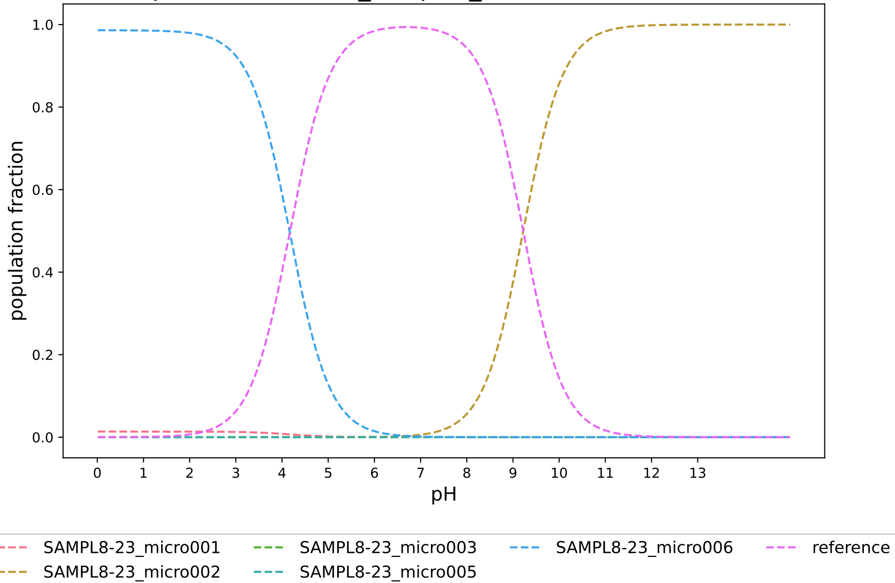
pKa-RobertRaddi_DeepGP_modified:SAMPL8-23
