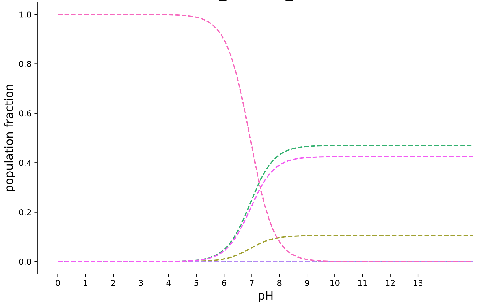
pKa-RobertRaddi_DeepGP_modified:SAMPL8-3
