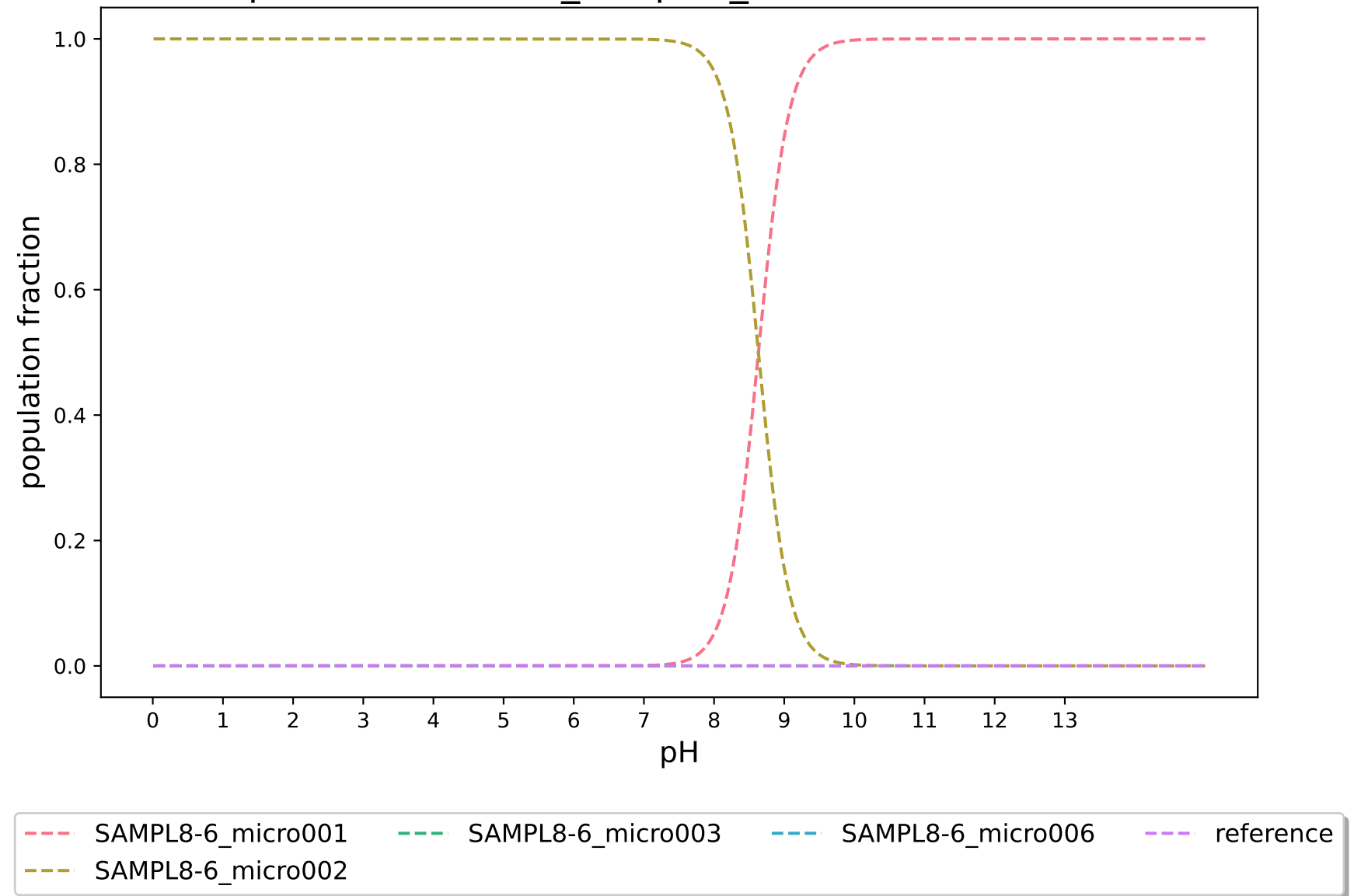
pKa-RobertRaddi_DeepGP_modified:SAMPL8-6
