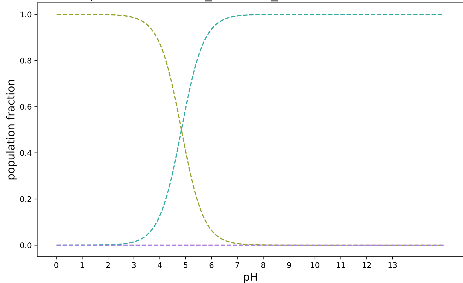
pKa-RobertRaddi_XGBoost_modified:SAMPL8-2
