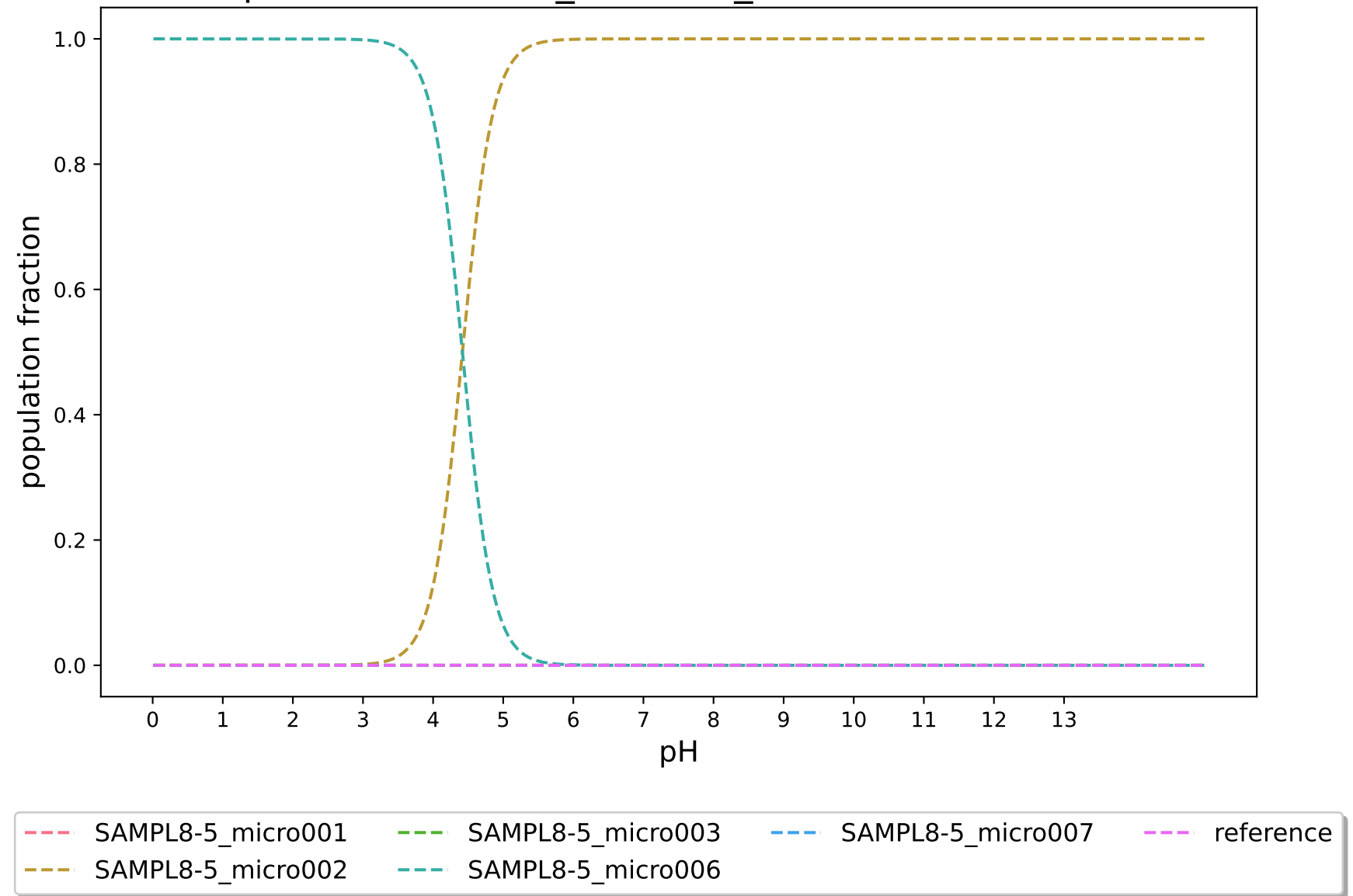
pKa-RobertRaddi_XGBoost_modified:SAMPL8-5
