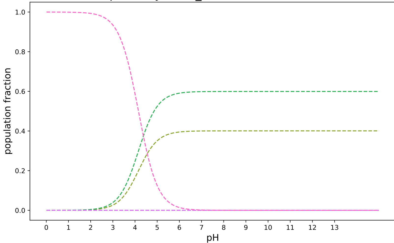
pKa-ZhiyiWu-1_modified:SAMPL8-1
