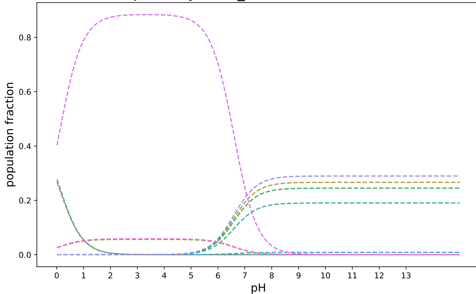
pKa-ZhiyiWu-1_modified:SAMPL8-4
