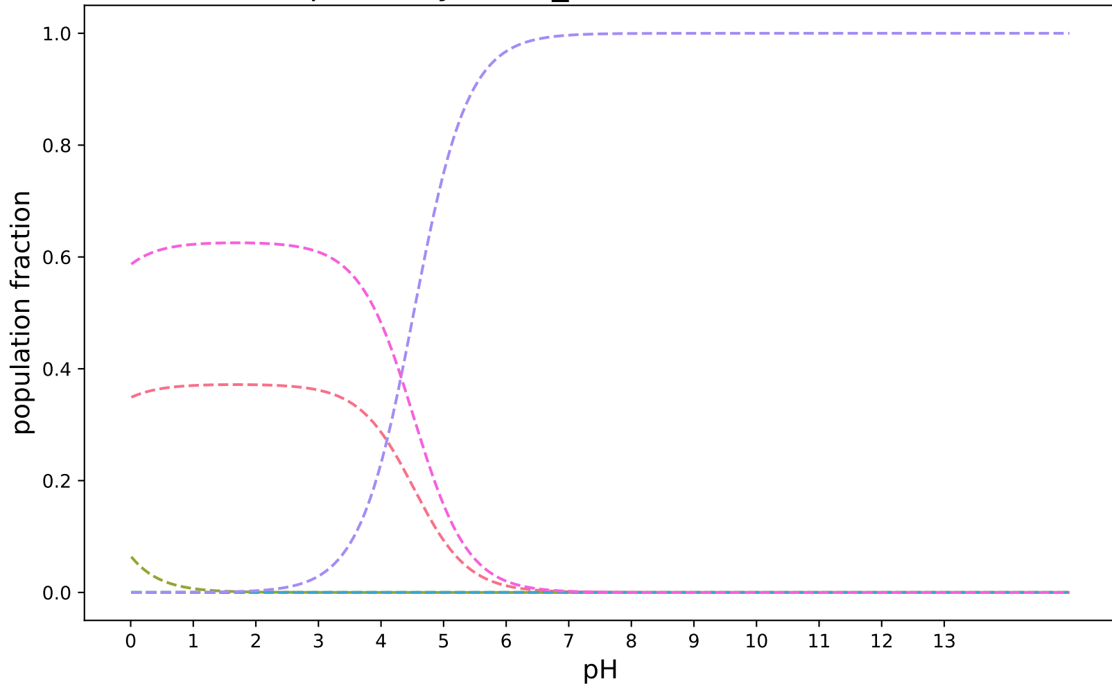
pKa-ZhiyiWu-1_modified:SAMPL8-5
