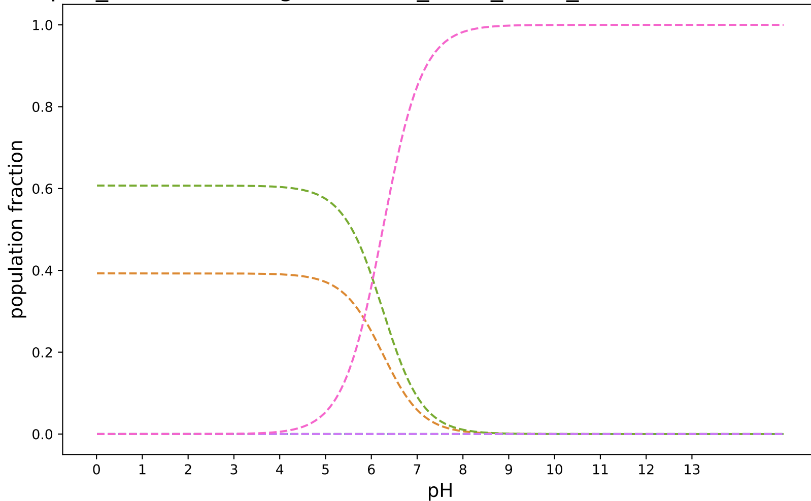
pKa_SabatinoRodriguezPaluch_uESE_extra_modified:SAMPL8-12
