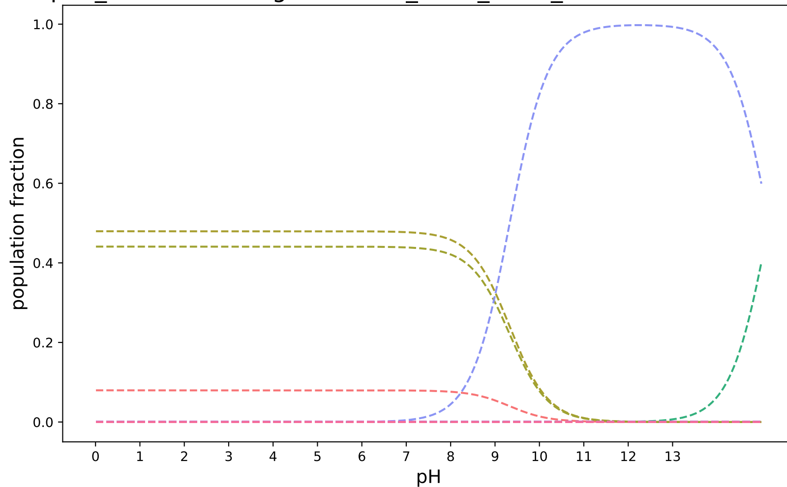
pKa_SabatinoRodriguezPaluch_uESE_extra_modified:SAMPL8-14
