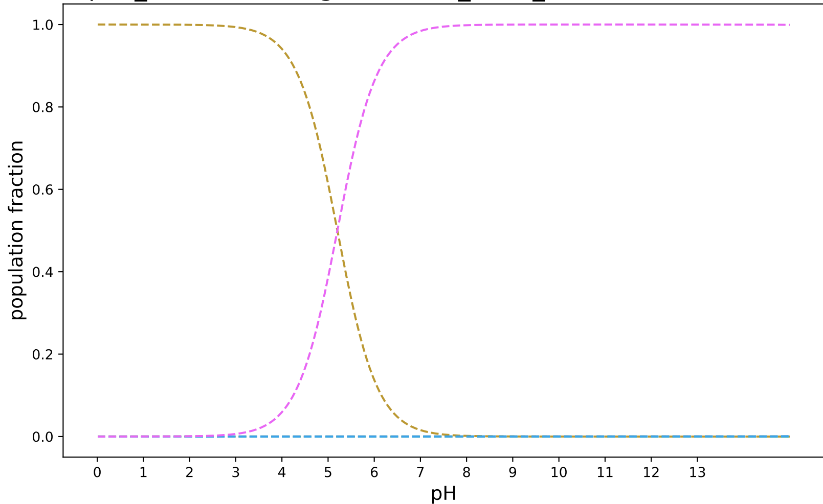
pKa_SabatinoRodriguezPaluch_uESE_modified:SAMPL8-17
