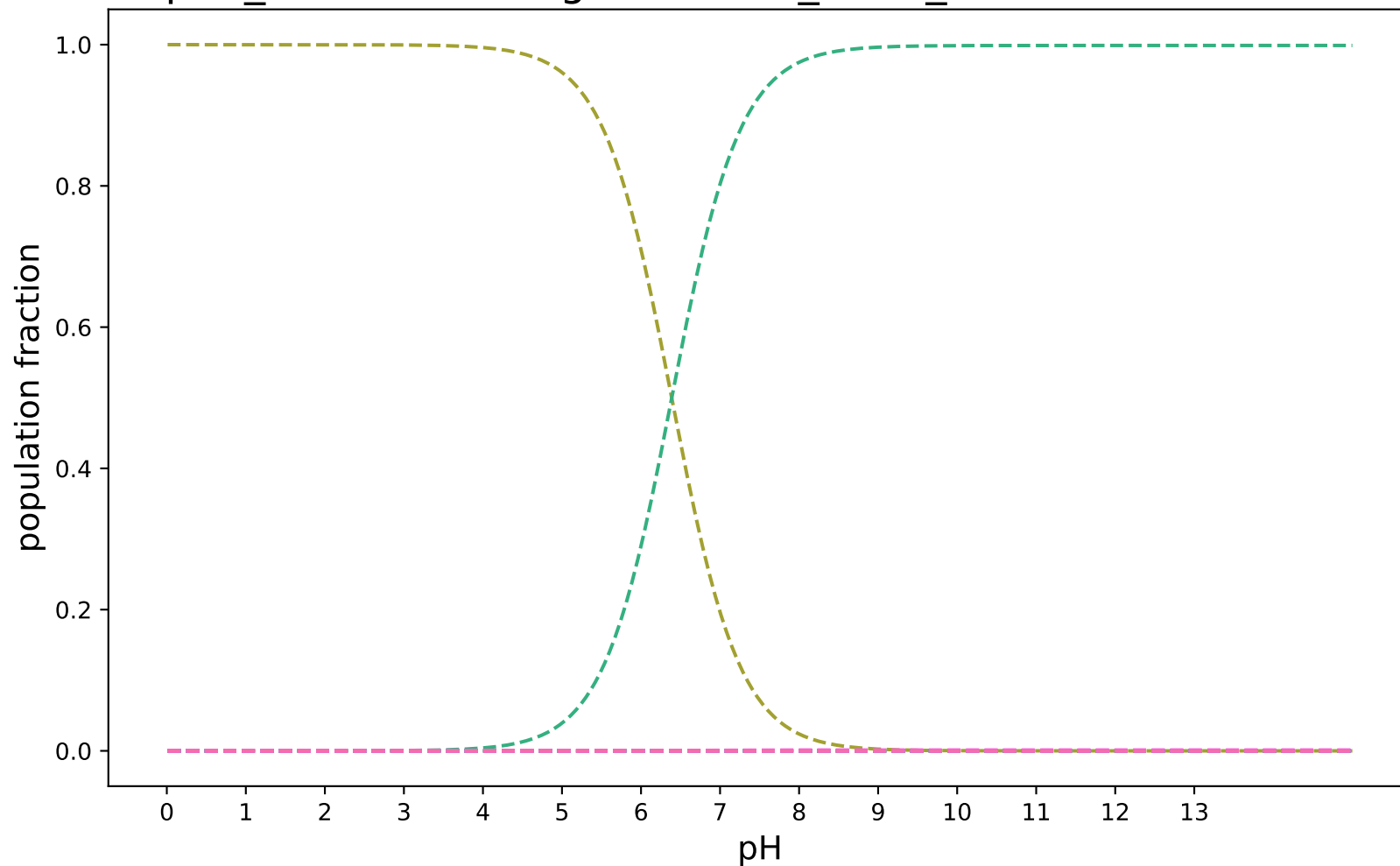
pKa_SabatinoRodriguezPaluch_uESE_modified:SAMPL8-3
