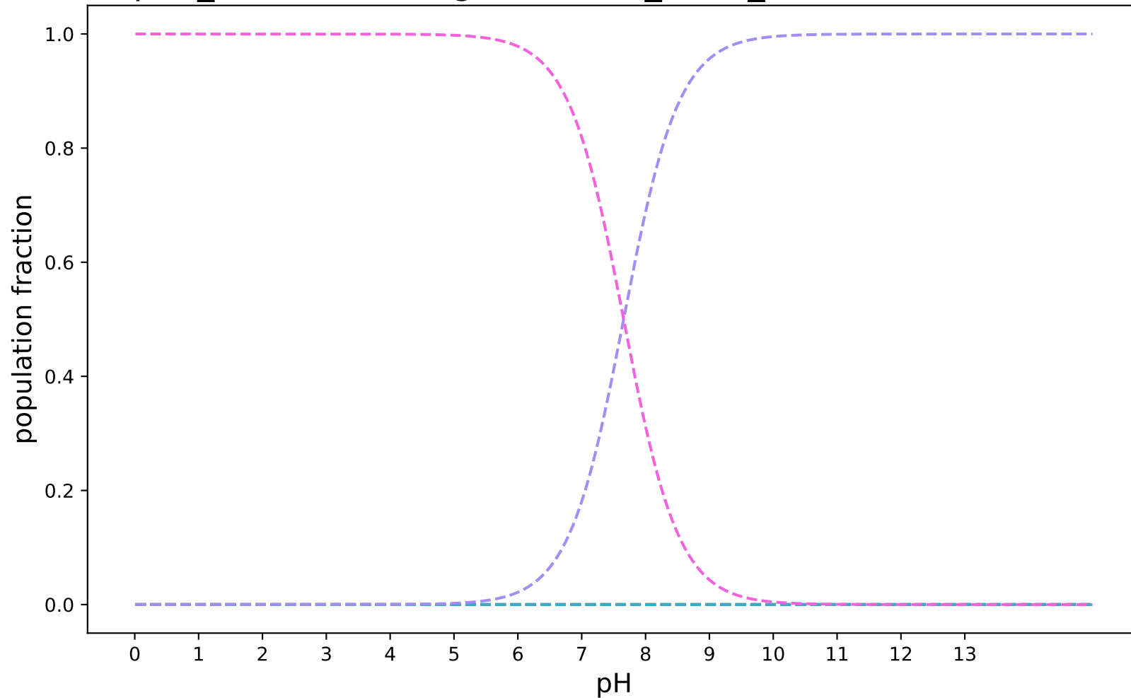
pKa_SabatinoRodriguezPaluch_uESE_modified:SAMPL8-5
