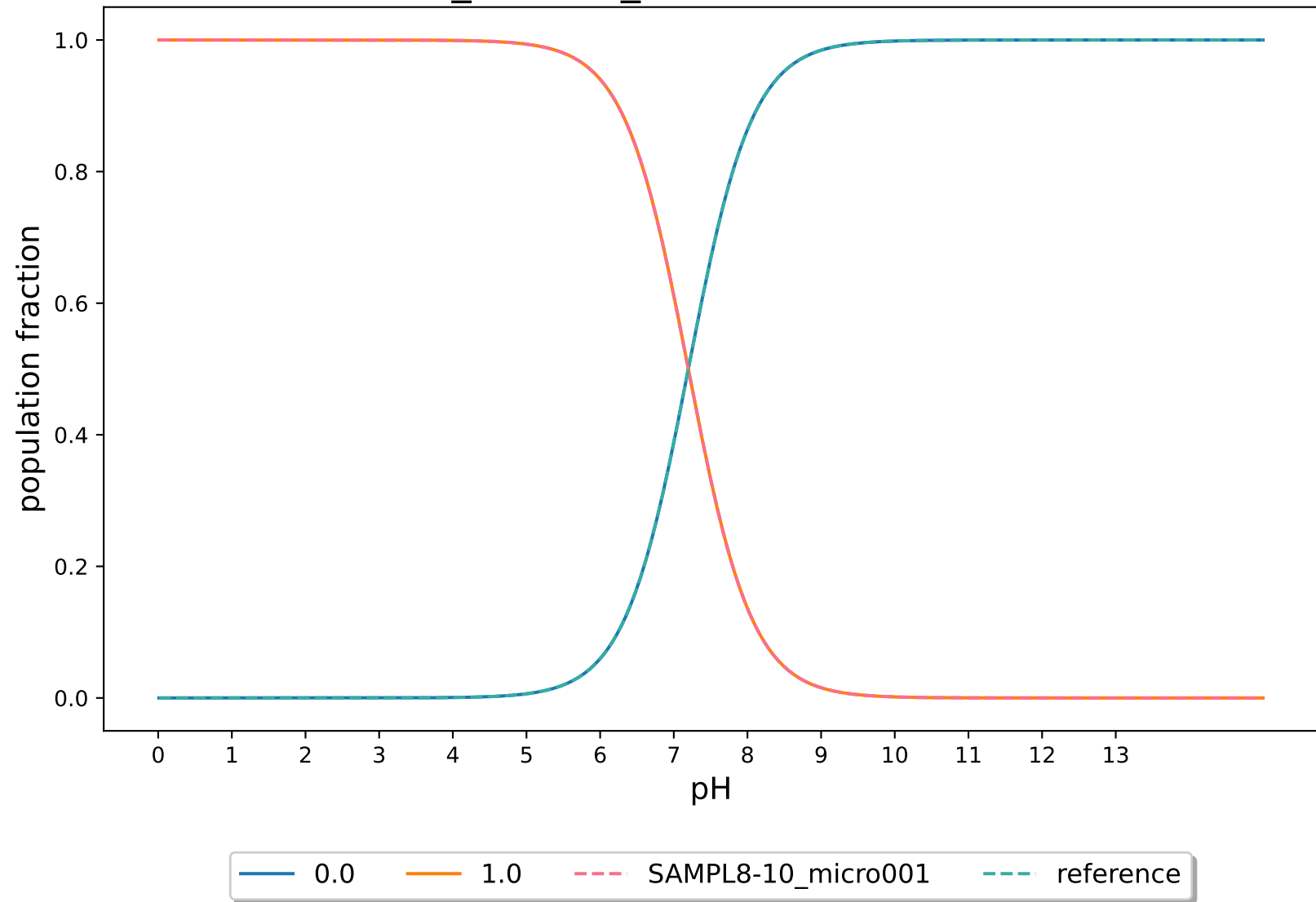
PKA_ECRISM_modified:SAMPL8-10
