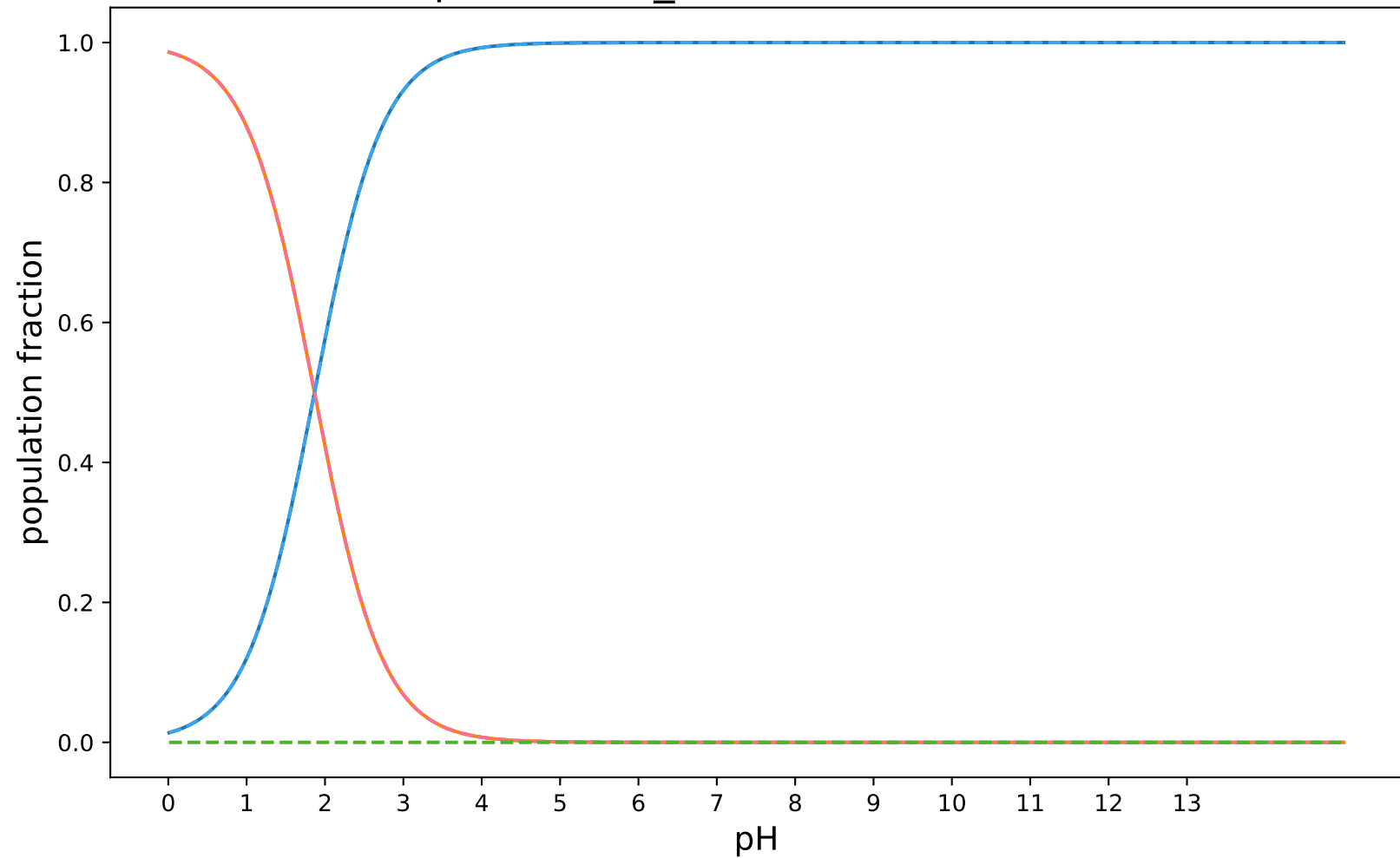
pKa-3DS-1_modified:SAMPL8-8
