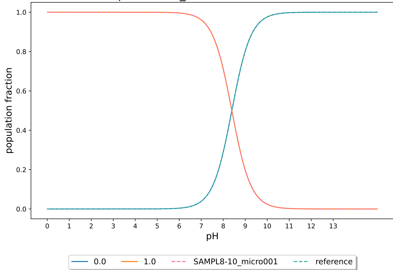
pKa-3DS-2_modified:SAMPL8-10
