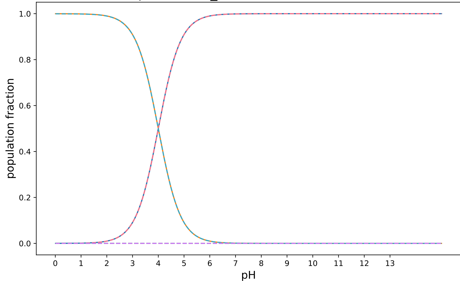
pKa-3DS-2_modified:SAMPL8-15
