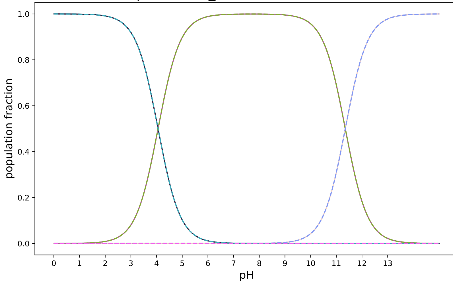
pKa-3DS-2_modified:SAMPL8-18
