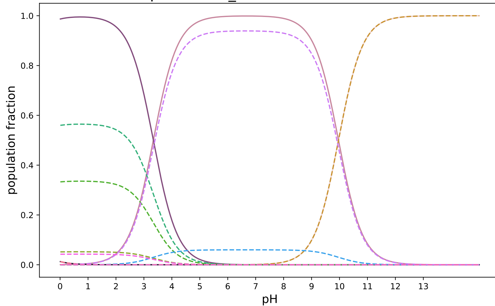
pKa-3DS-2_modified:SAMPL8-20
