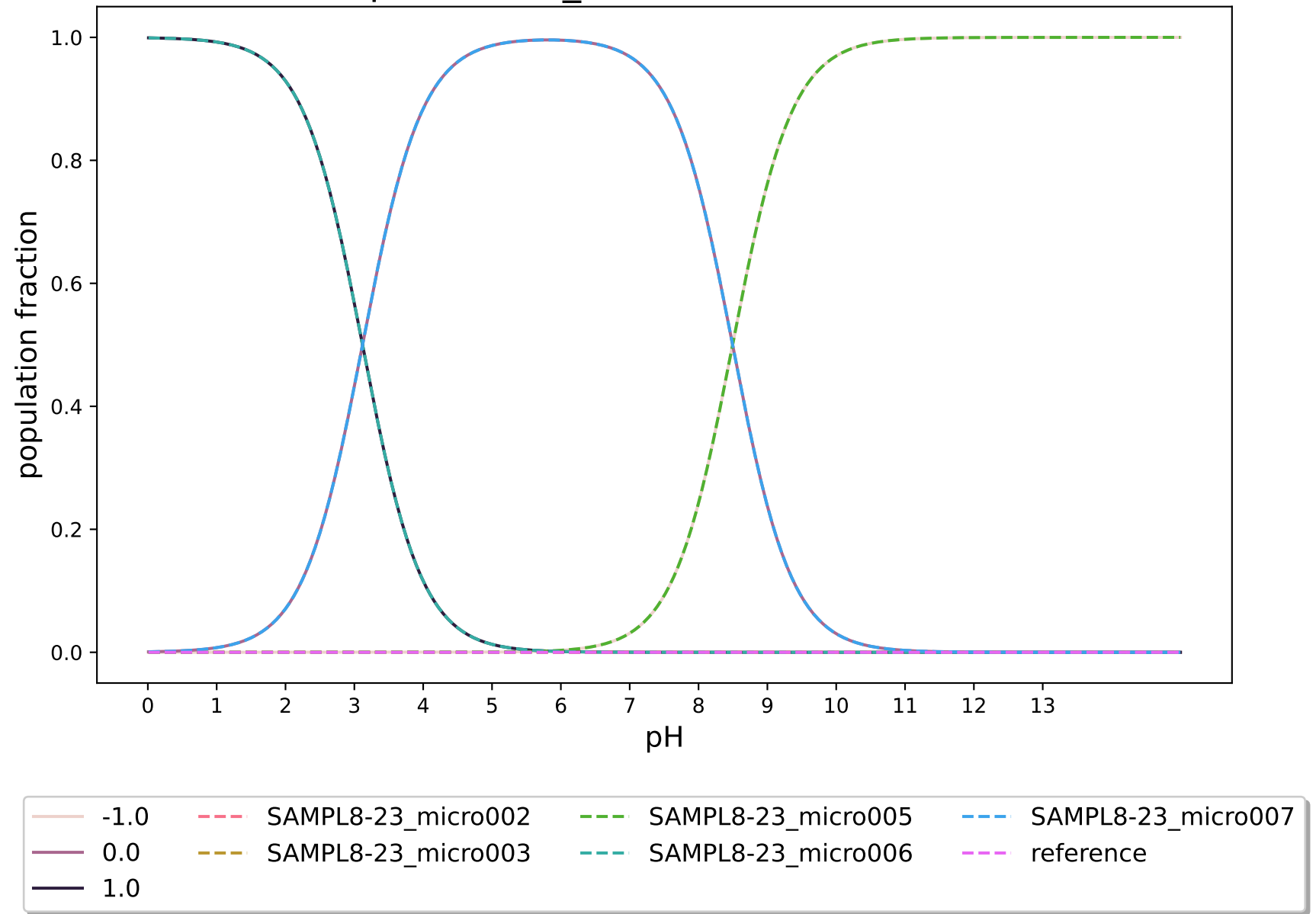
pKa-3DS-2_modified:SAMPL8-23
