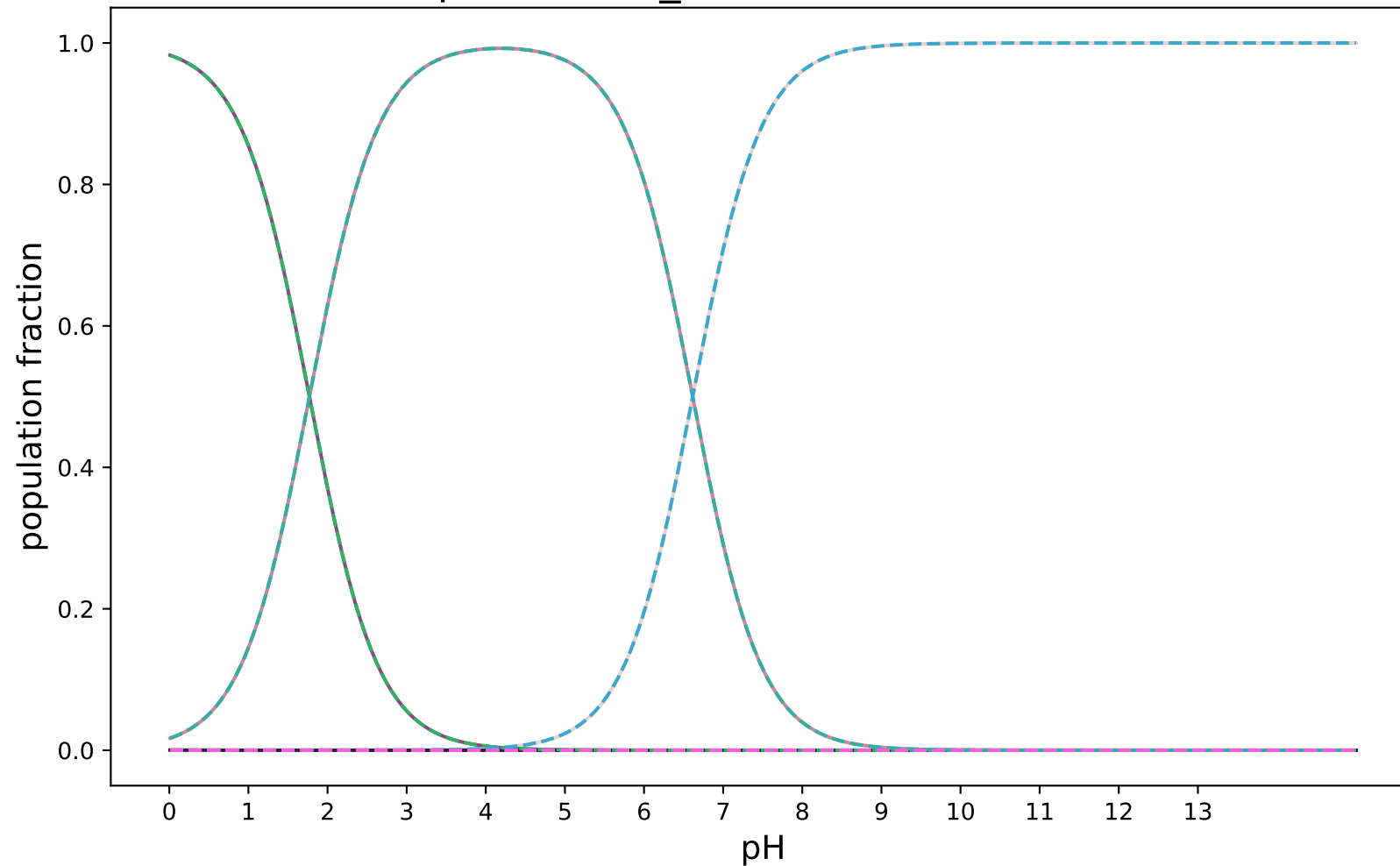
pKa-3DS-2_modified:SAMPL8-3
