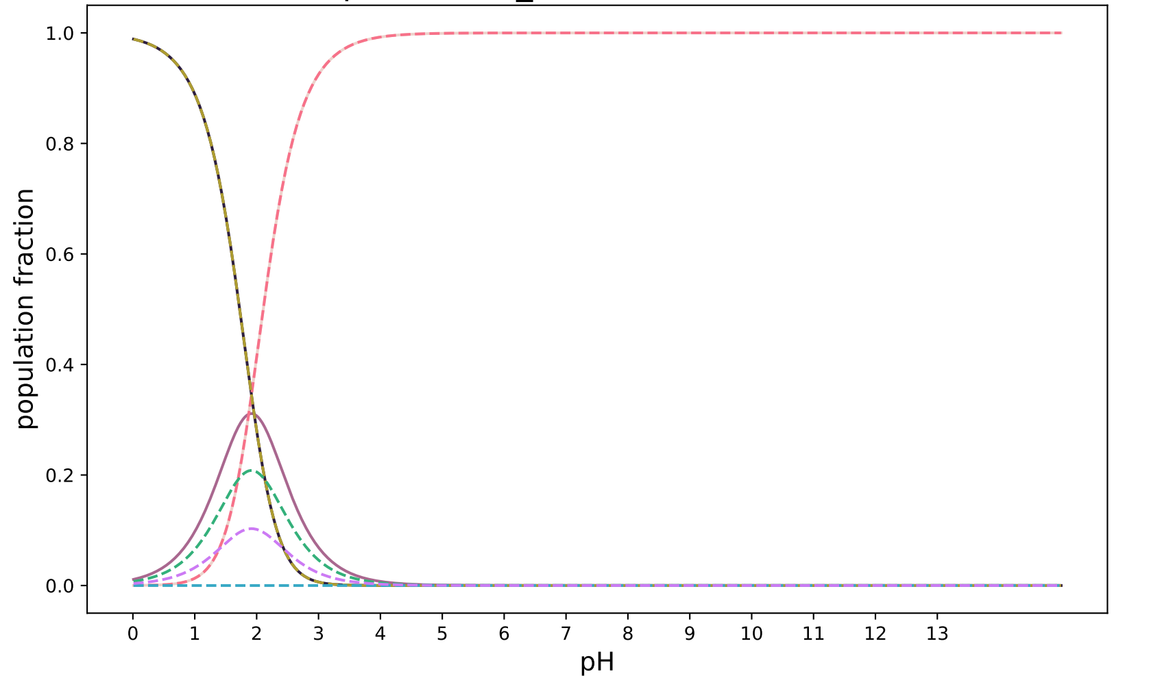
pKa-3DS-2_modified:SAMPL8-6
