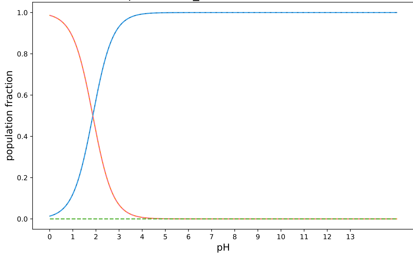
pKa-3DS-2_modified:SAMPL8-8
