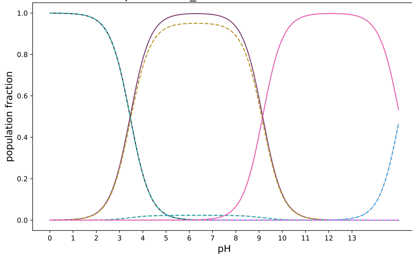
pKa-3DS-3_modified:SAMPL8-12
