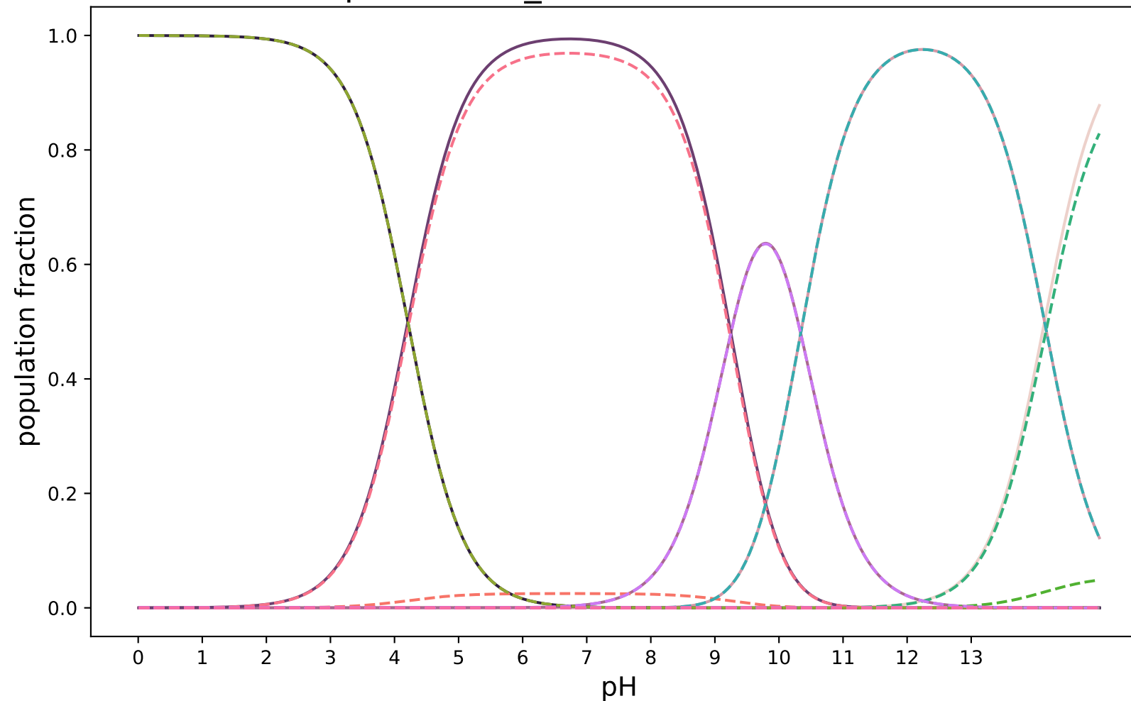
pKa-3DS-3_modified:SAMPL8-14
