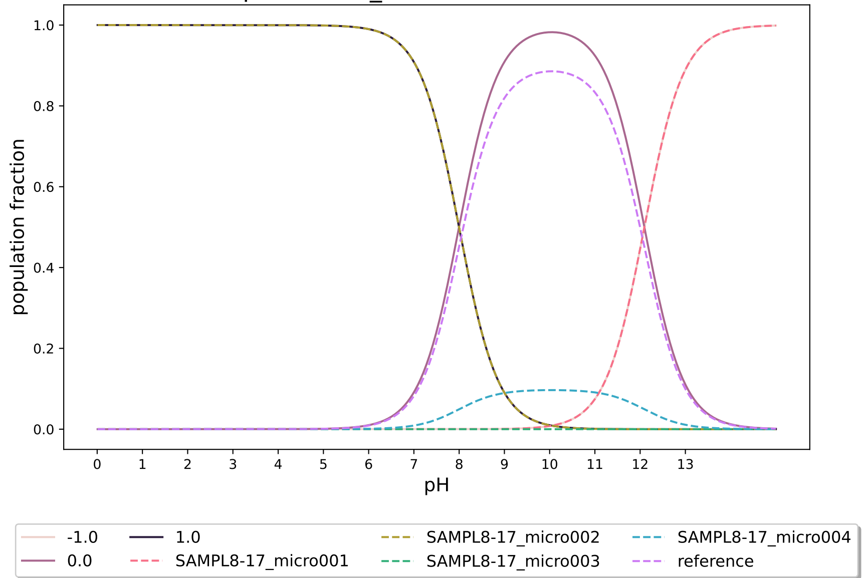
pKa-3DS-3_modified:SAMPL8-17
