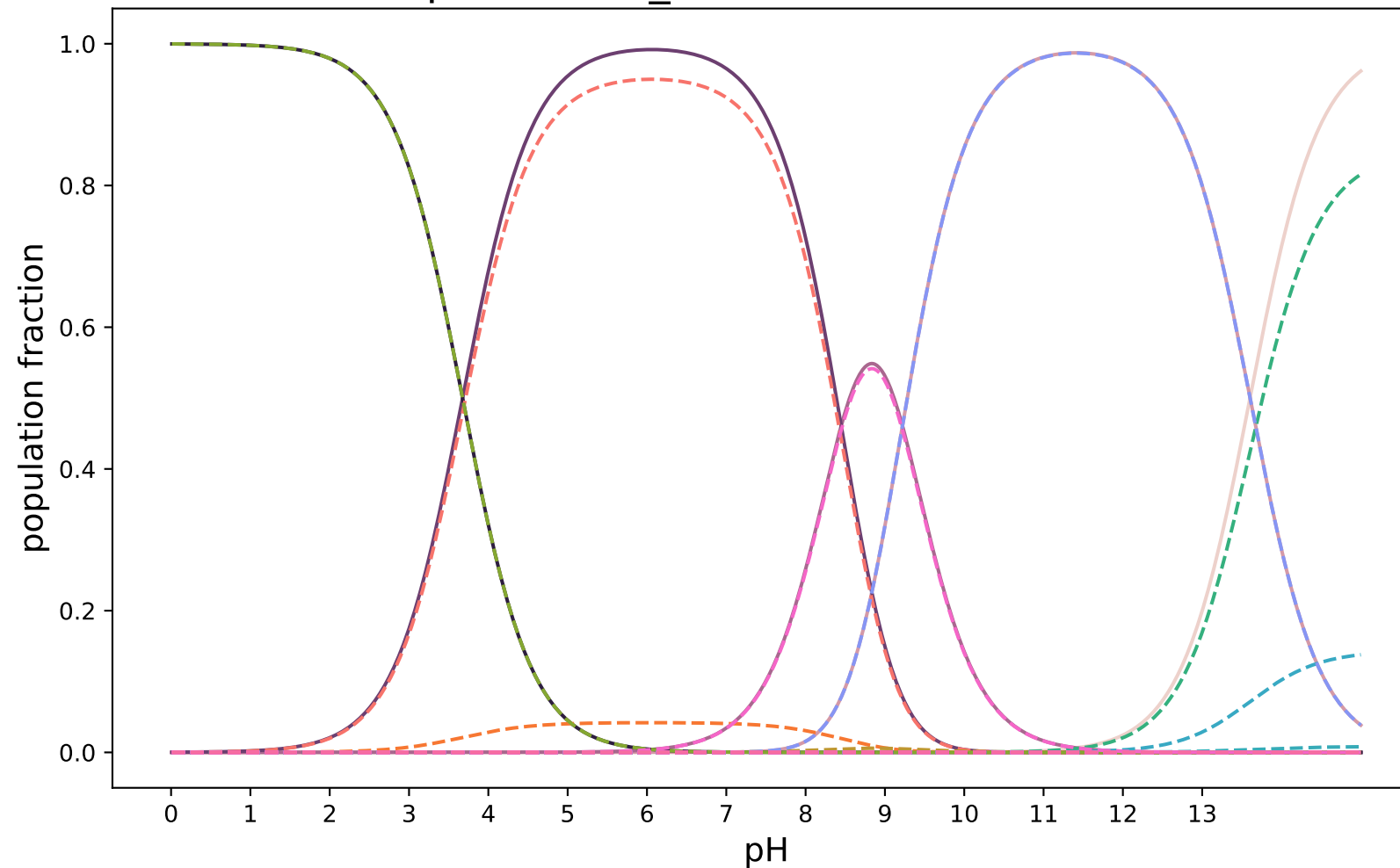
pKa-3DS-3_modified:SAMPL8-21
