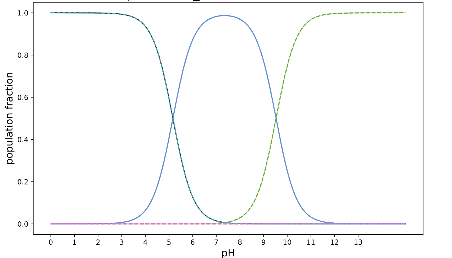
pKa-3DS-3_modified:SAMPL8-23
