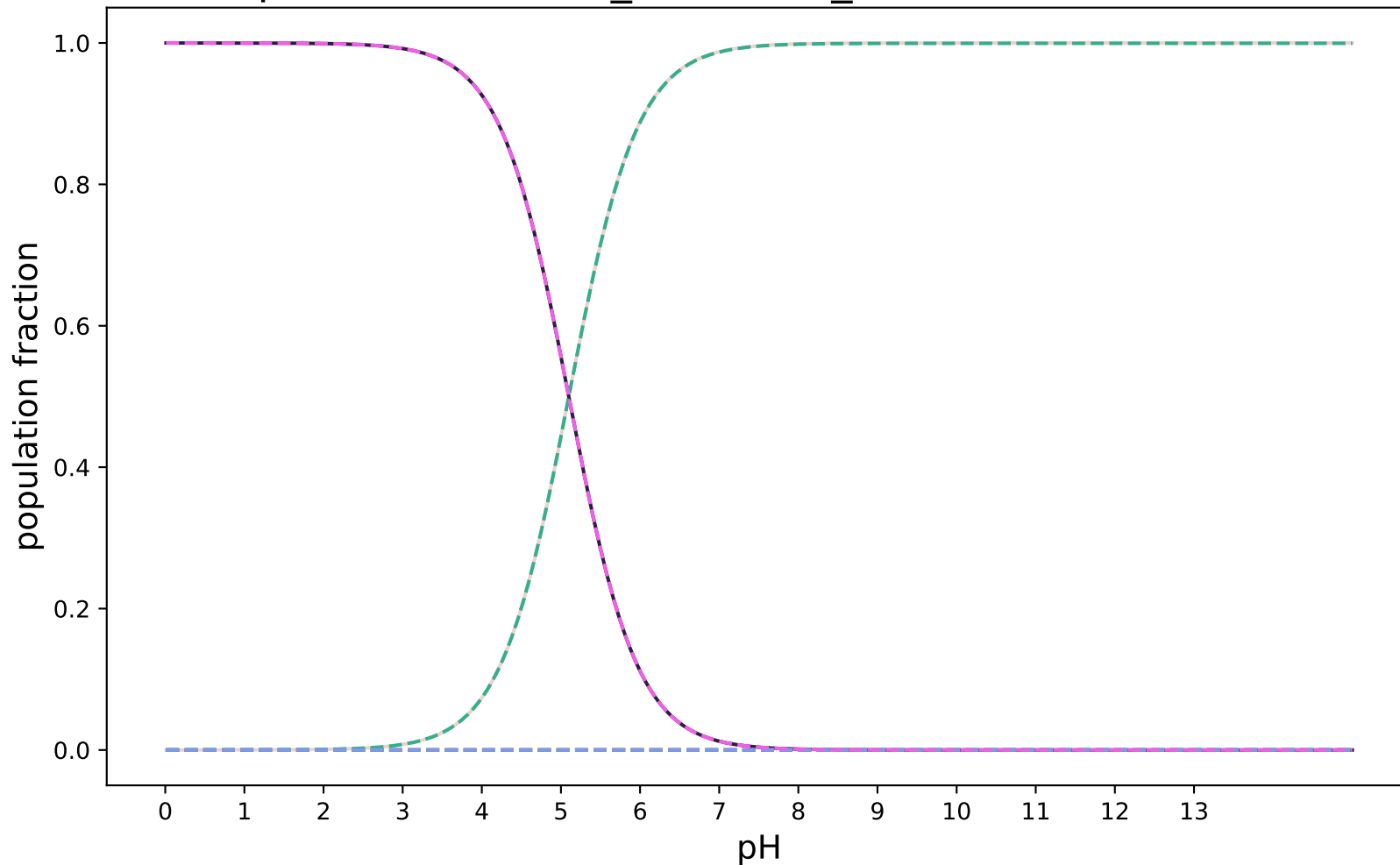
pKa-RobertRaddi_AdaBoost_modified:SAMPL8-1
