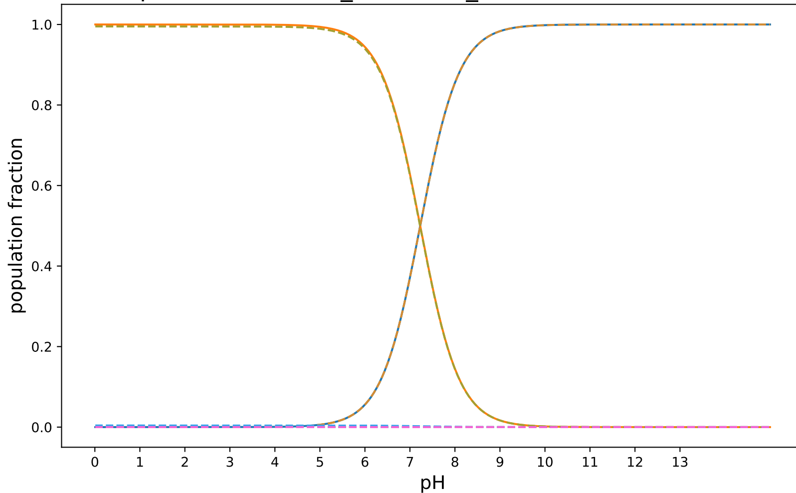
pKa-RobertRaddi_AdaBoost_modified:SAMPL8-16
