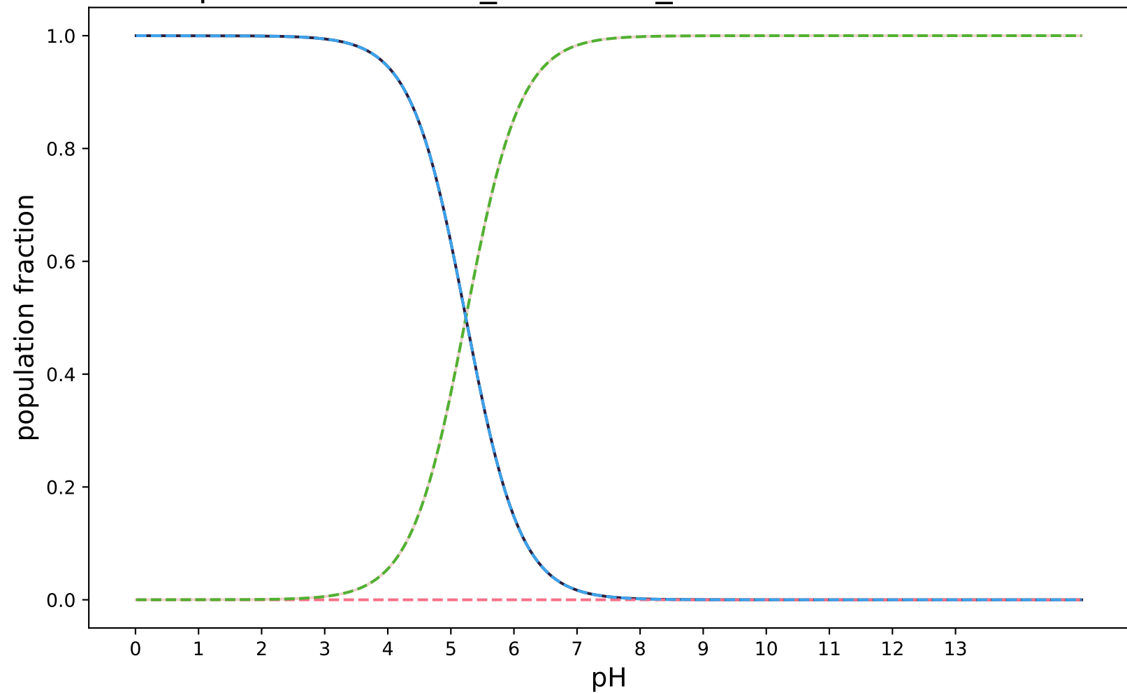
pKa-RobertRaddi_AdaBoost_modified:SAMPL8-17
